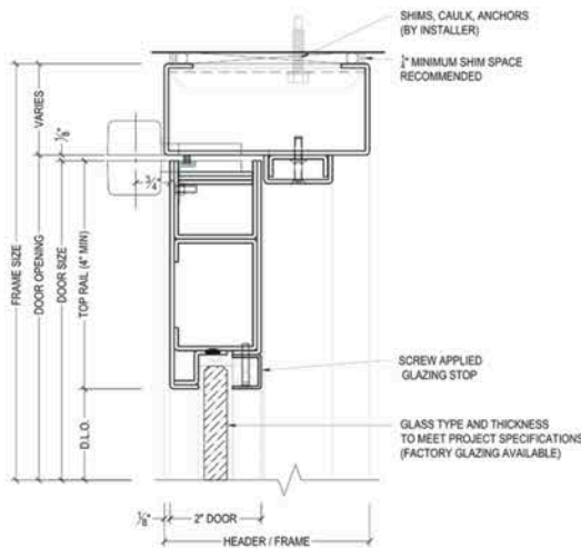
HEADER / TOP RAIL
