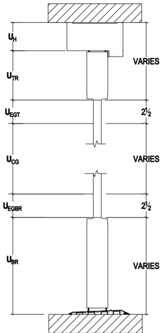
Figure 6: Component Section View Taken Along a Vertical Section Line
