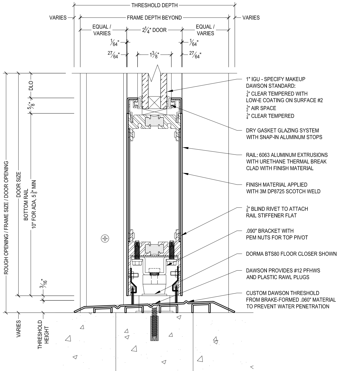
3 BOTTOM RAIL @ CLOSER Scale: 1:2
